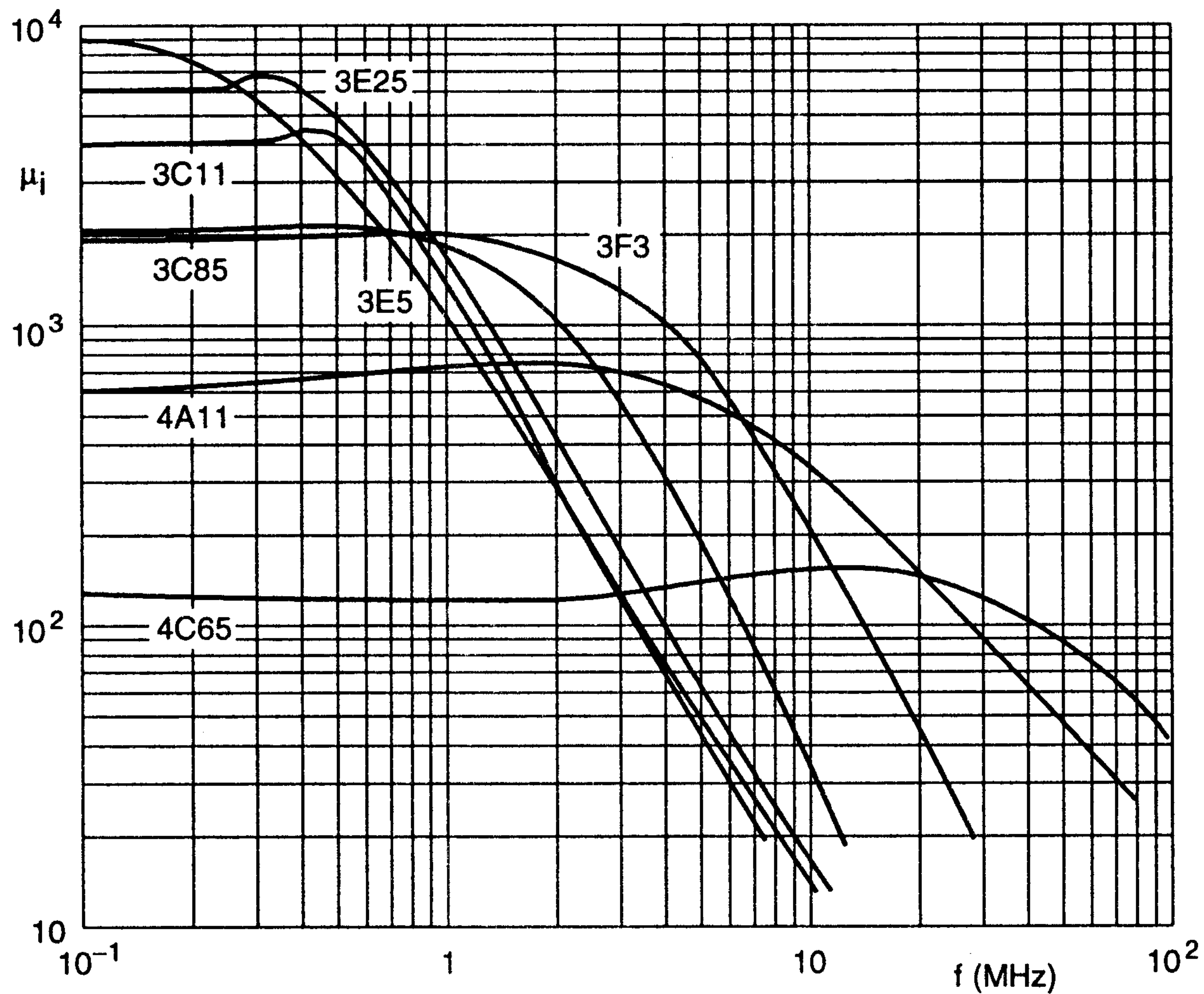
Permeability as a function of frequency of different material grades.
